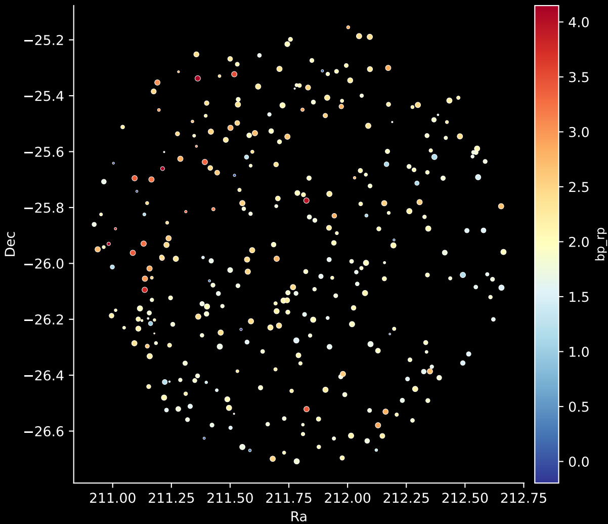
APOGEE DR17 Field: [240-04] Stars: 317
