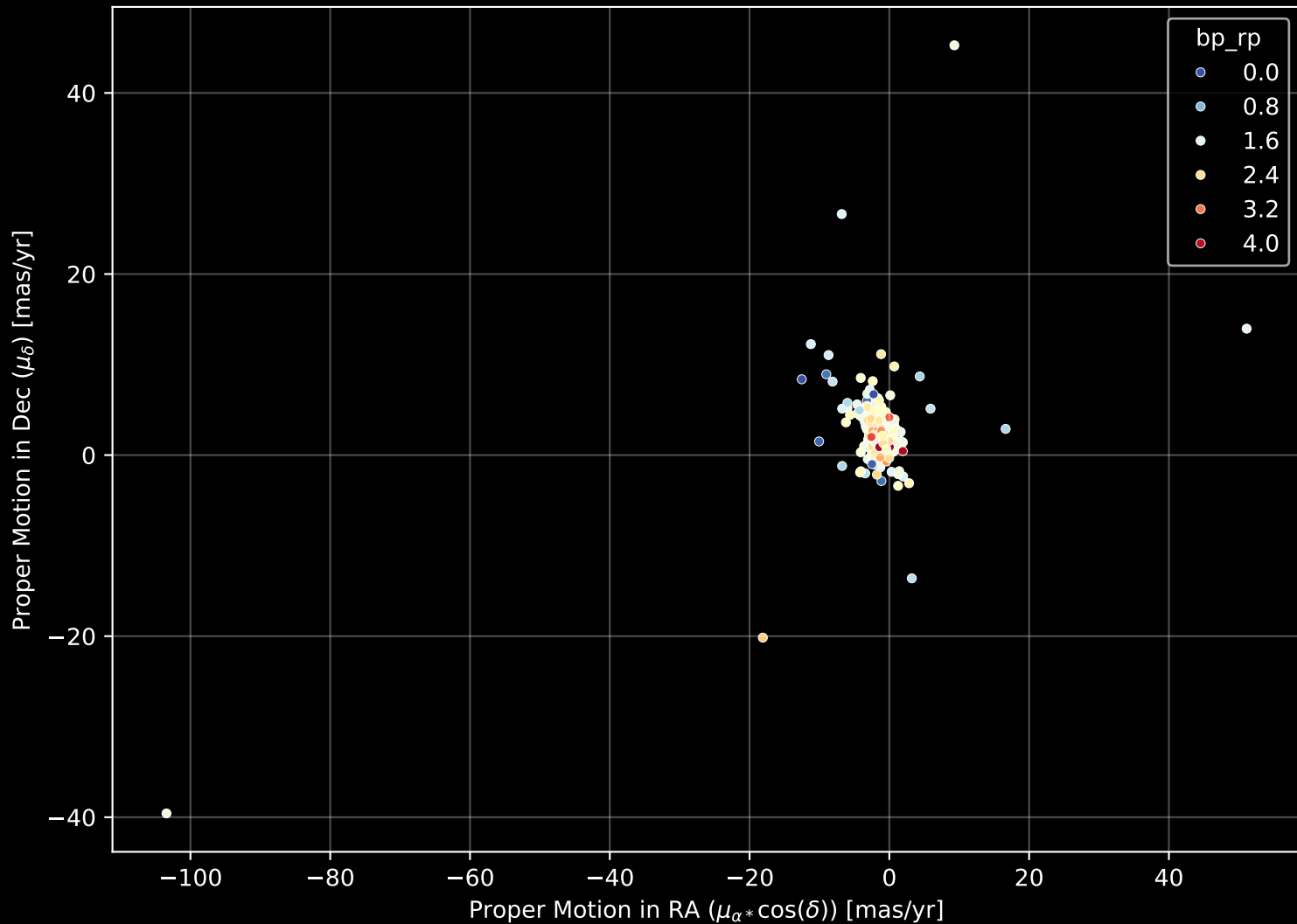
APOGEE DR17 Field: [240-04] Proper Motion Diagram (n= 317)
