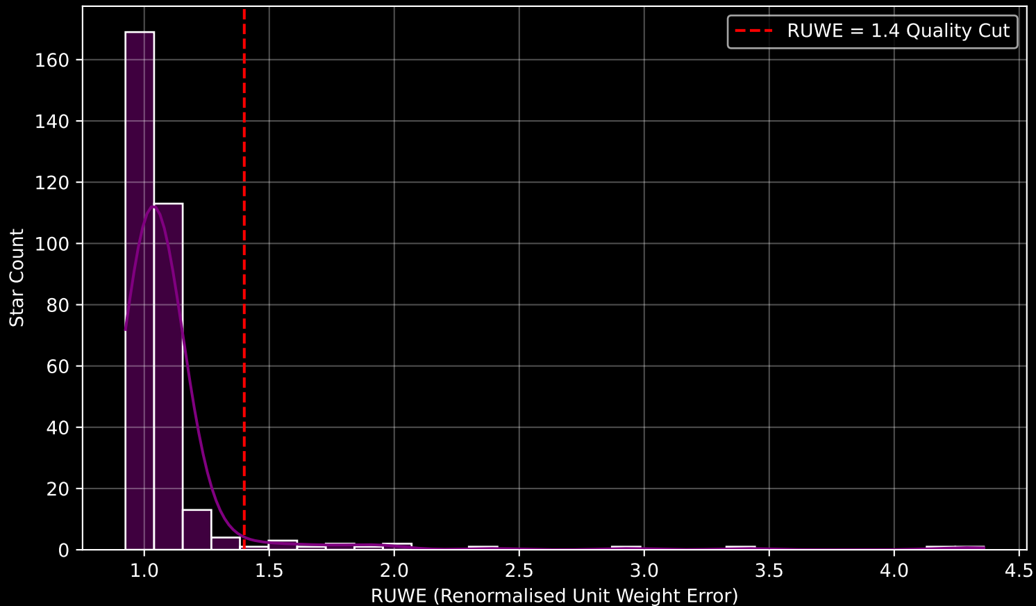
GAPOGEE DR17 Field [240-04] RUWE Distribution (n= 314)
