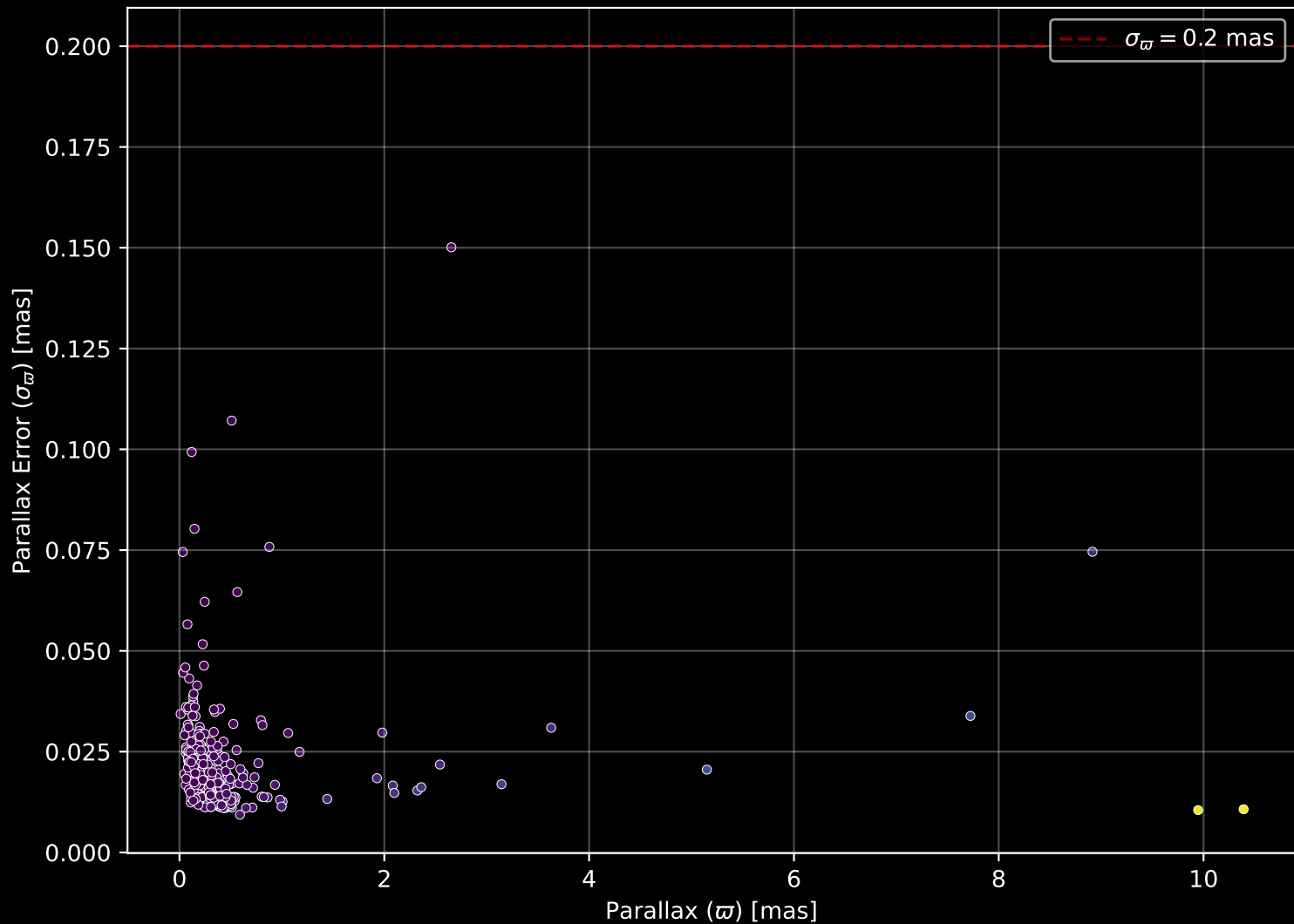
APOGEE DR17 Field: [240-04] Parallax Quality (n= 317)
