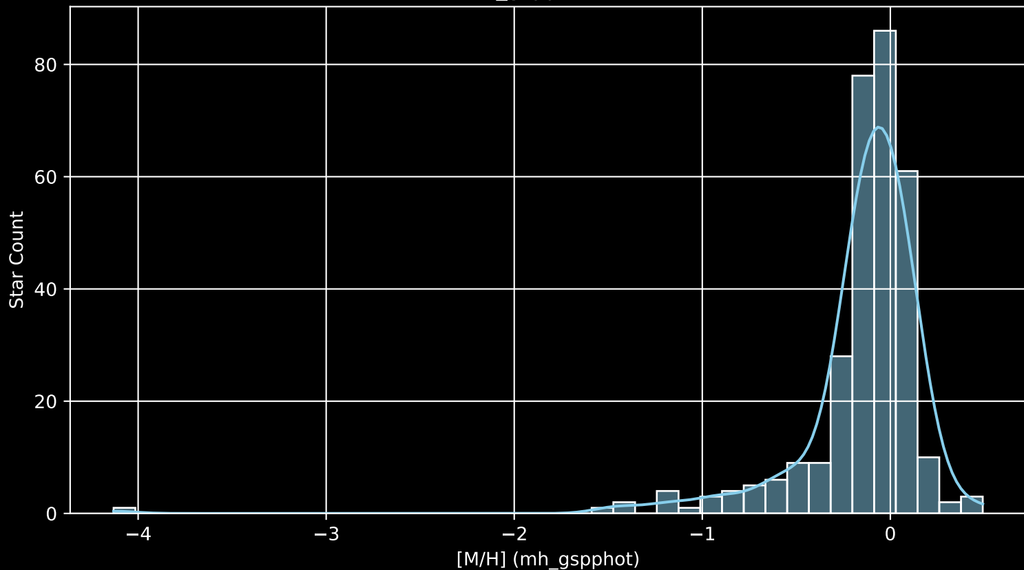
APOGEE DR17 Field: [240-04 [M/H] (mh_gspphot) (n= 313)
